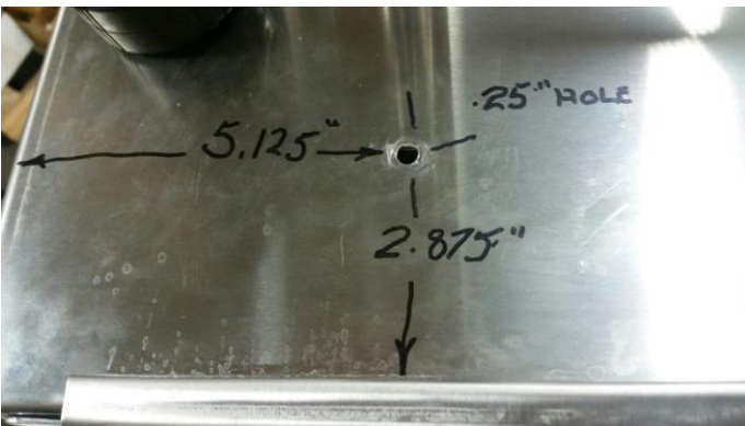
Drill a hole in the top of the hood on the left hand side, 5.125" from back, 2.875" from side of hood Hole is for a 1/4" bolt, use a 9/32 (.281") drill for easier fit, seal bolt with flat washer.
